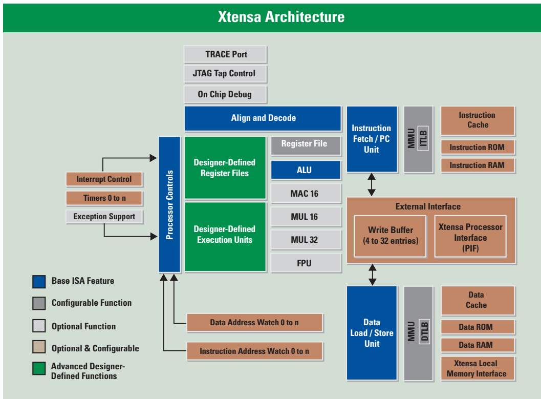
Figure 1: The Xtensa architecture consists of various configurable building blocks. CONFIGURABLE FUNCTION blocks are elements parameterized by the system designer. OPTIONAL FUNCTION blocks indicate elements available to accelerate specific applications. OPTIONAL AND CONFIGURABLE blocks are optional elements scalable to fit applications, including peripherals. ADVANCED DESIGNER-DEFINED FUNCTIONS are hardware execution units and registers added to the processor by the designer to accelerate specific algorithms for a given SOC design. Common in all configurations is the base instruction set architecture.
